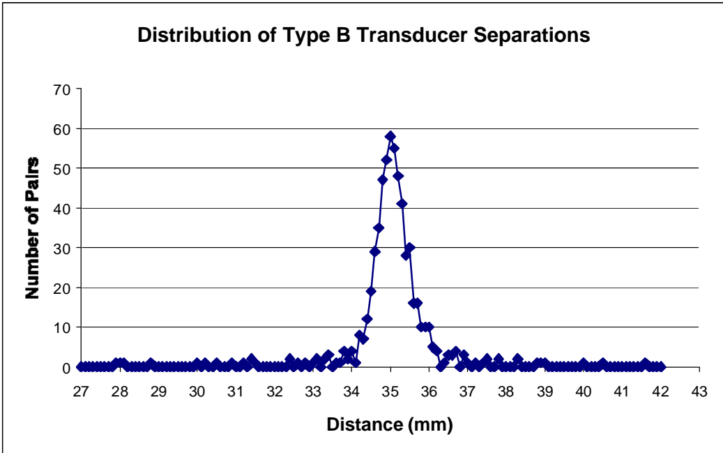
Figure 3. Distribution of measured separations for 603 pairs of Type B transducers designed for use on ASL's new ASFM Advantage instrument.
