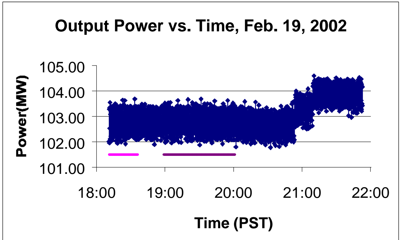
Figure 6. Turbine power output during the February 19, 2002 transducer spacing measurements at Lower Monumental Dam. The plotted points represent results of power measurements at 10 s intervals. Solid lines positioned below the plotted data denote the 18:11-18:36 and 18:59-20:01 time intervals used to obtain time delay data for, respectively, Type A and Type B transducers.
