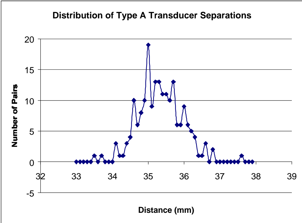
Figure 2. Distribution of measured separations for 190 pairs of Type A transducers used on ASL's in-house early ASFM instrument.
