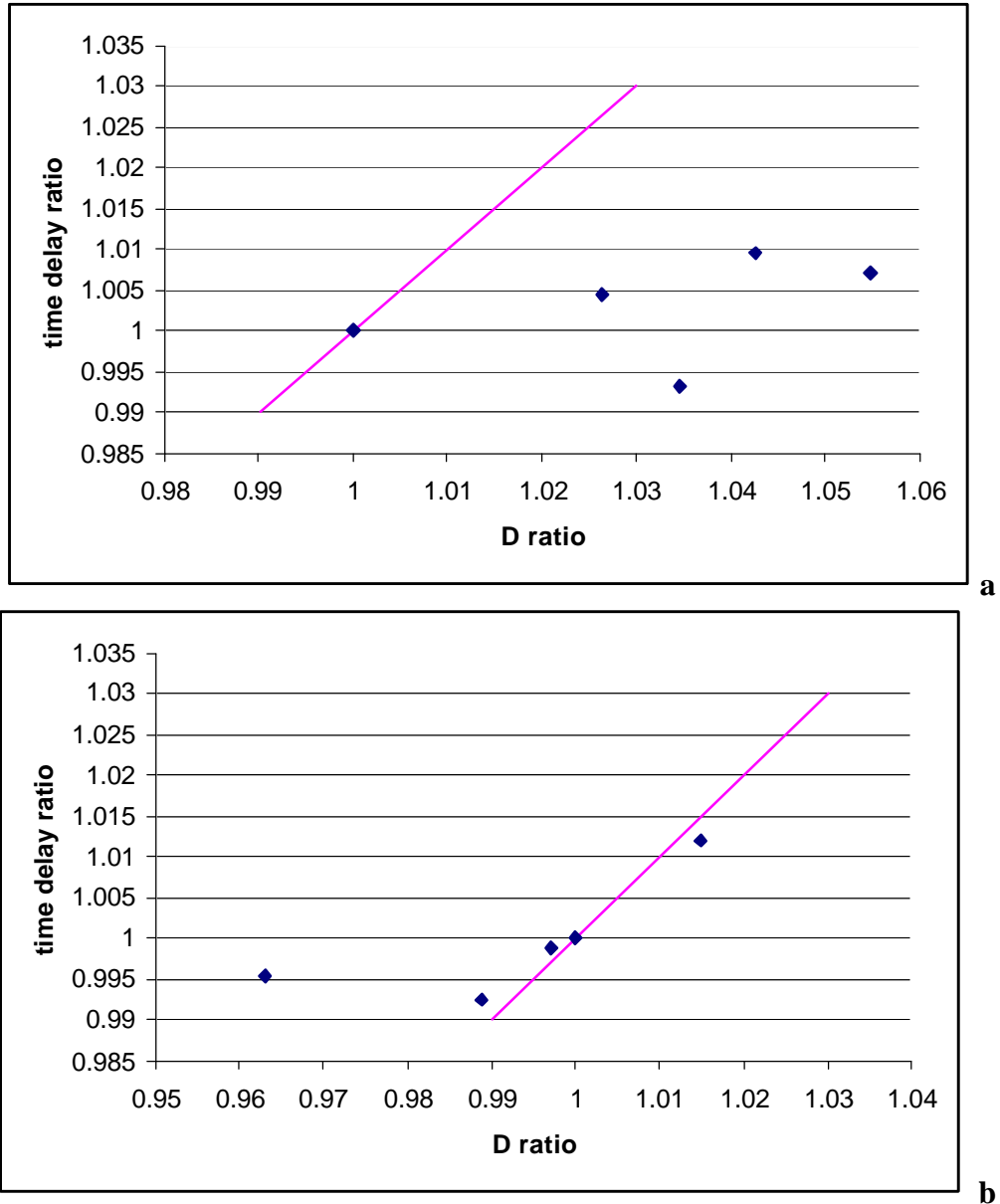
Figure 5. Plots of the measured (on January 21, 2002) ratios of time delays (vertical axes) on all measurement lines across the a) horizontal and b) diagonal transducer pairs (all relative to the time delay on line 5) as a function of the corresponding ratios (horizontal axes) of the acoustically measured mean transmitter + receiver spacings, D_{hi} and D_{di} . The included straight lines are representative of expectations assuming exact correspondence between the spacings implied by the flow-measured time delays and the mean spacing parameters, D_{hi} and D_{di} , derived from the acoustically measured spacings.
