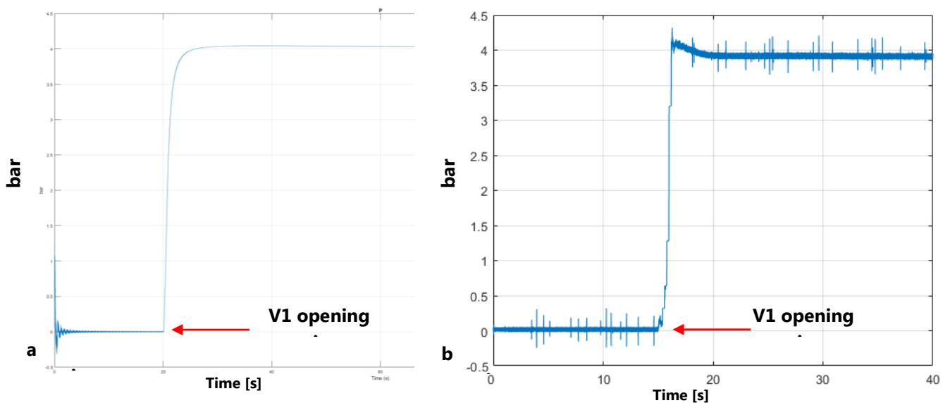
Fig. 7a-b: Pressure behavior computed from simulations (7a) and from in situ measurements (7b).
