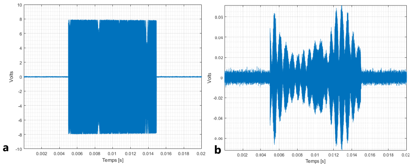
Fig. 6a depicts the ultrasonic signal emitted while Fig. 6b shows the received signal, which has been attenuated by the flow, such attenuation is related to the flow intrinsic characteristics.
