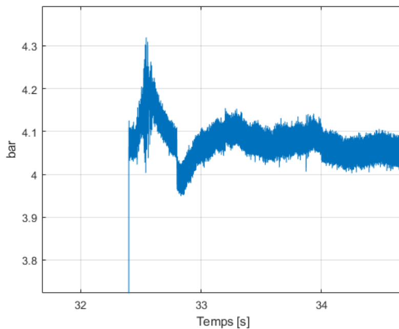
Fig. 8 shows a detailed view of the pressure peak and pressure fluctuation after the opening of V1
