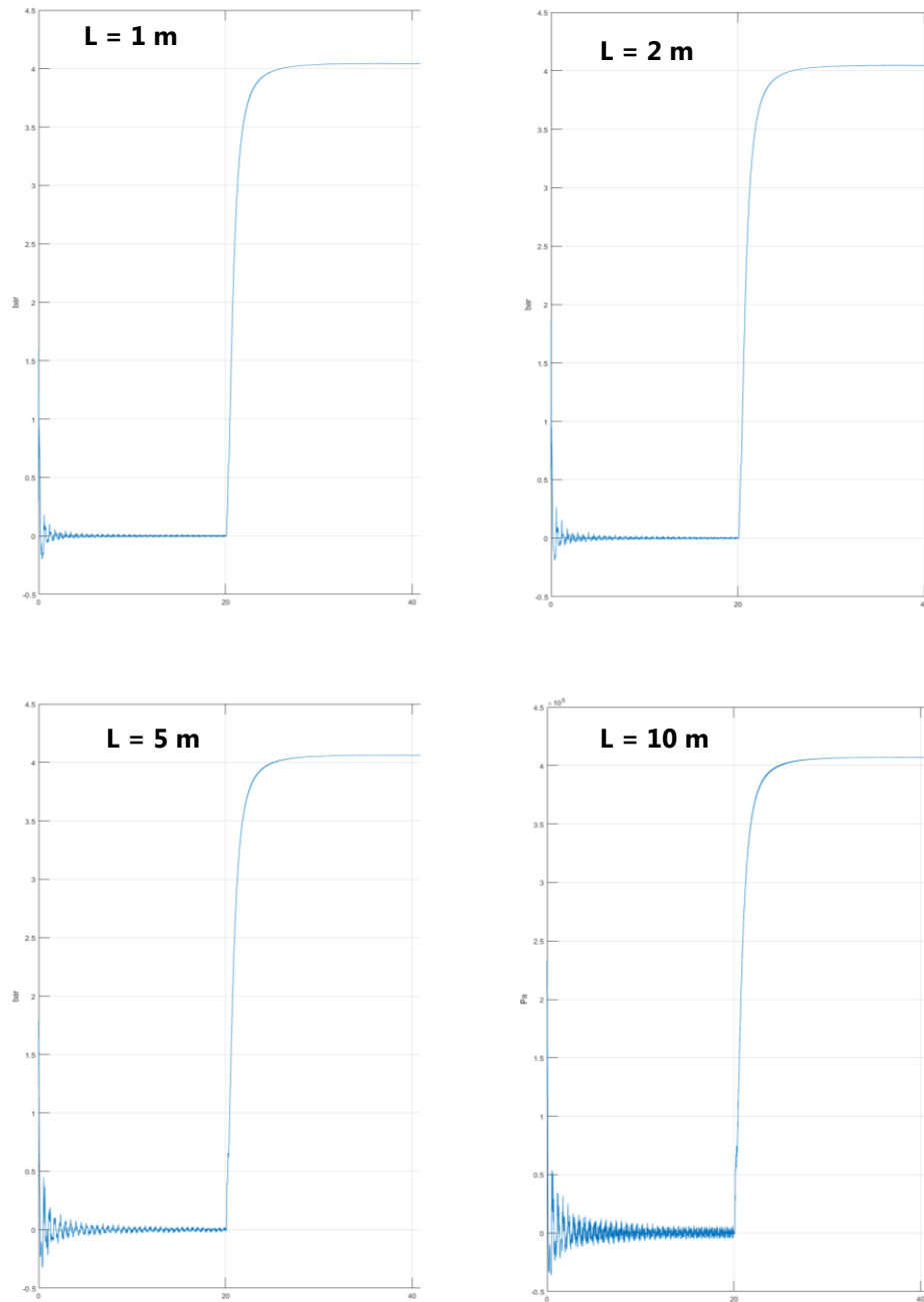
Fig. 11 shows different results of pressure behavior of iterations ranging from 1m to 10m regarding the location of the flow disturbance (valve V2).
