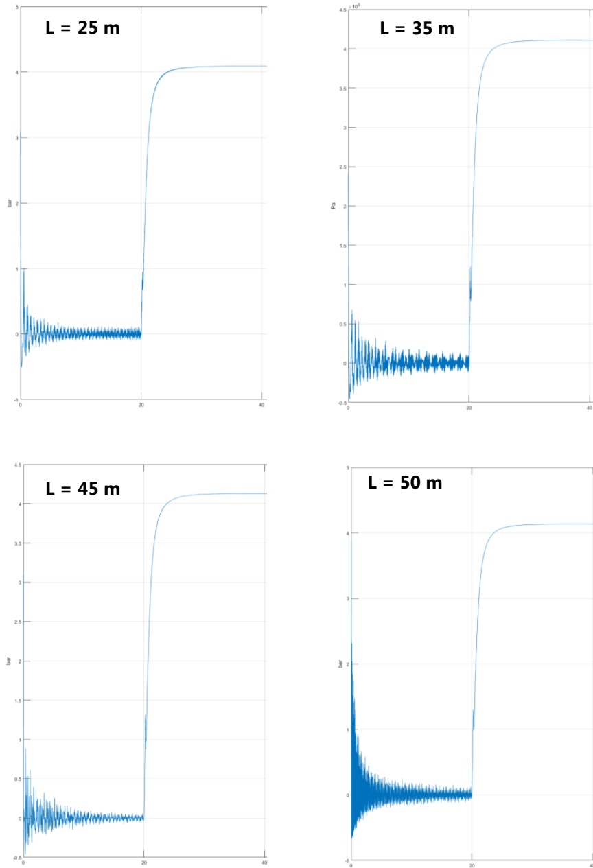
Fig. 12 shows different results of pressure behavior of iterations ranging from 25m to 50m regarding the location of the flow disturbance (valve V2).
