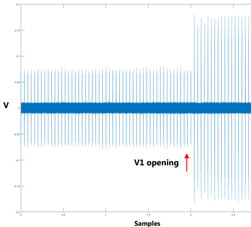
Fig. 10 zoomed-in the region when the valve is opened, it shows no important attenuation after the valve is opened since there is no vapour present due valve V1 cavitating, because cavitation bubbles already collapsed upstream
