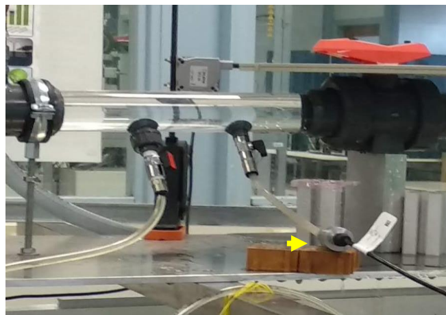
Fig. 4 depicts the pressure sensor (signalled by the yellow arrow) which is installed 10 cm before valve V2;
