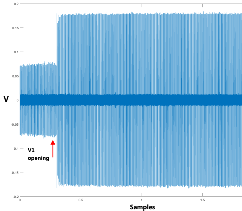
Fig. 9 depicts the development of the ultrasonic signal received before, during and after the opening of valve V1
