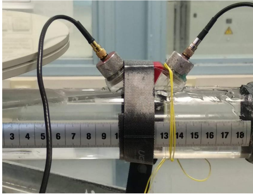
Fig. 5 shows the ultrasonic transducers installed downstream the valve V2. They are installed in a “V” configuration, which means the ultrasonic beam bounces off from the inner wall of the pipe to the ultrasonic receiver performing a “V” trajectory.
